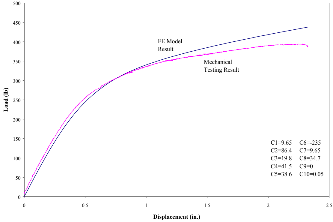
Fig. 4-26 Load-Displacement Curves of a 5 Foot Long Beam with 4 Foot Span and Load Applied at 1/3 of the Span (User-Supplied Material 2)
