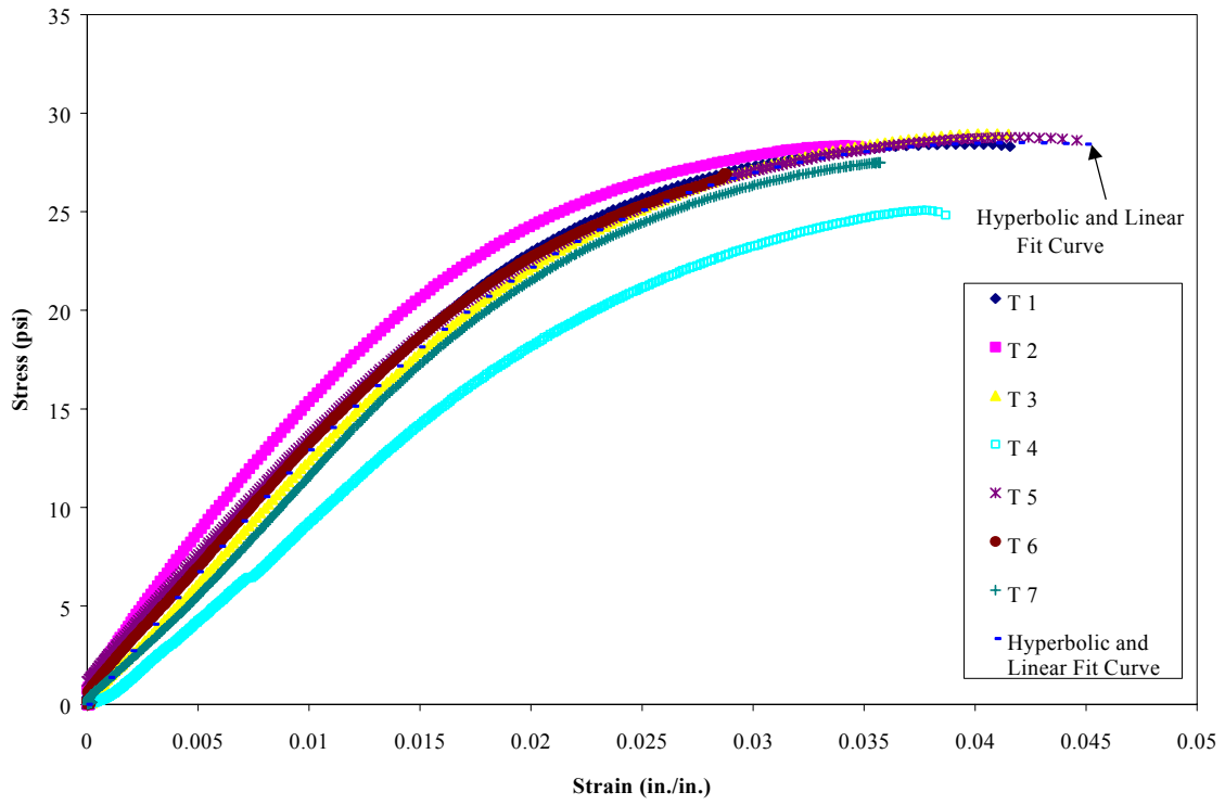
Fig. 4-5 Stress-Strain Curves for EPS in Tension between Testing & Hyperbolic and Linear Function Fit
