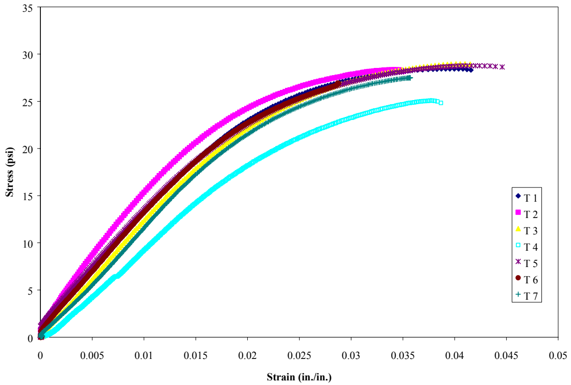
Fig. 4-4 Stress-Strain Curves for EPS in Tension
