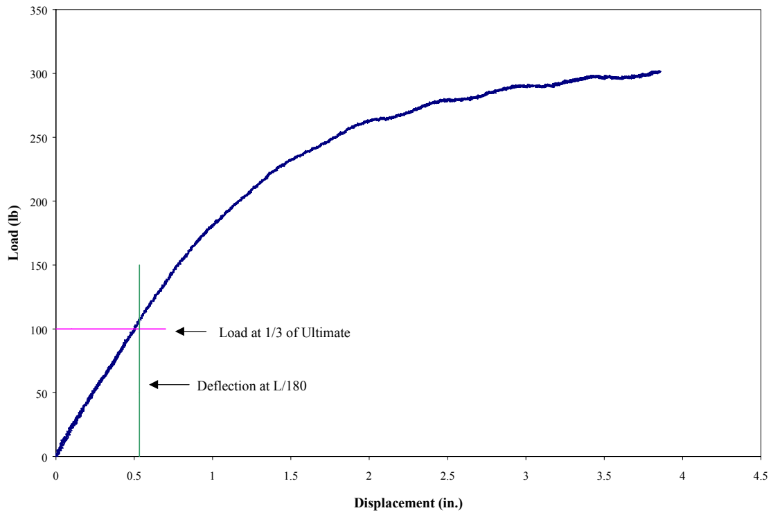
Fig. 5-7 Design Point for an 8 Foot Long Beam Provided by APA
