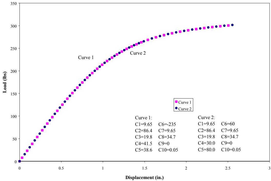
Fig. 5-3 Comparison of Load-Displacement Curves with Different Input for Tension Properties
