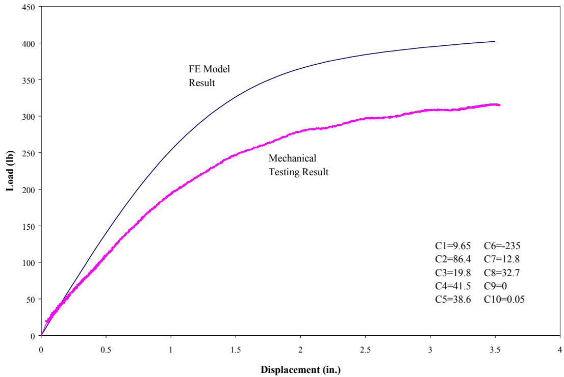
Fig. 4-24 Load-Displacement Curves of an 8 Foot Long Beam with 8 Foot Span and Load Applied at 1/3 of the Span (User-Supplied Material 1)
