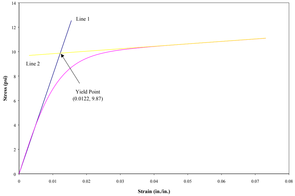
Fig. 4-3 EPS Continuous Point for Compression
