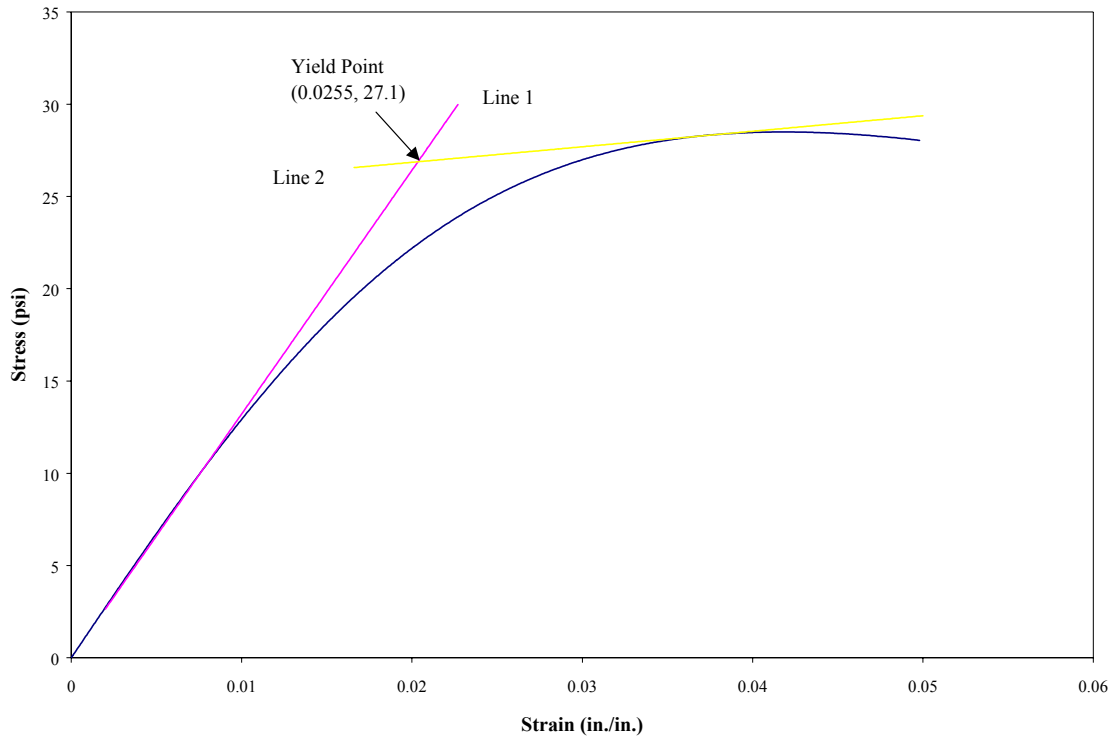
Fig. 4-6 EPS Discontinuous Point for Tension
