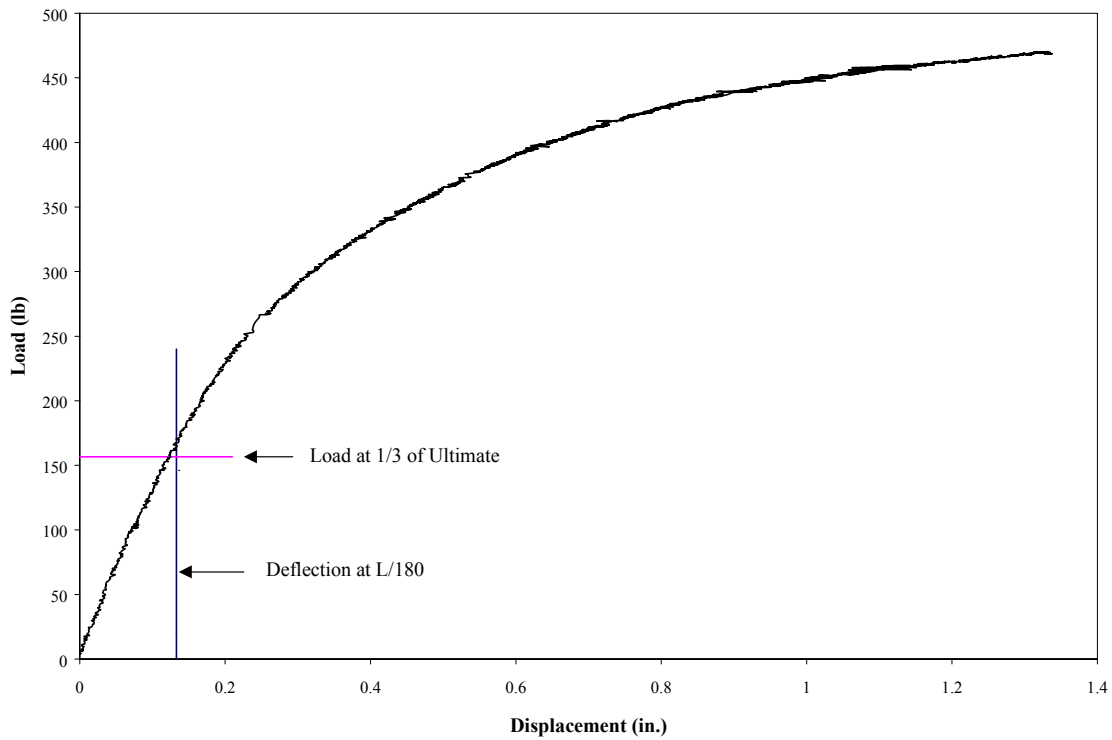
Fig. 5-4 Design Point for a 3 Foot Long Beam Provided by APA
