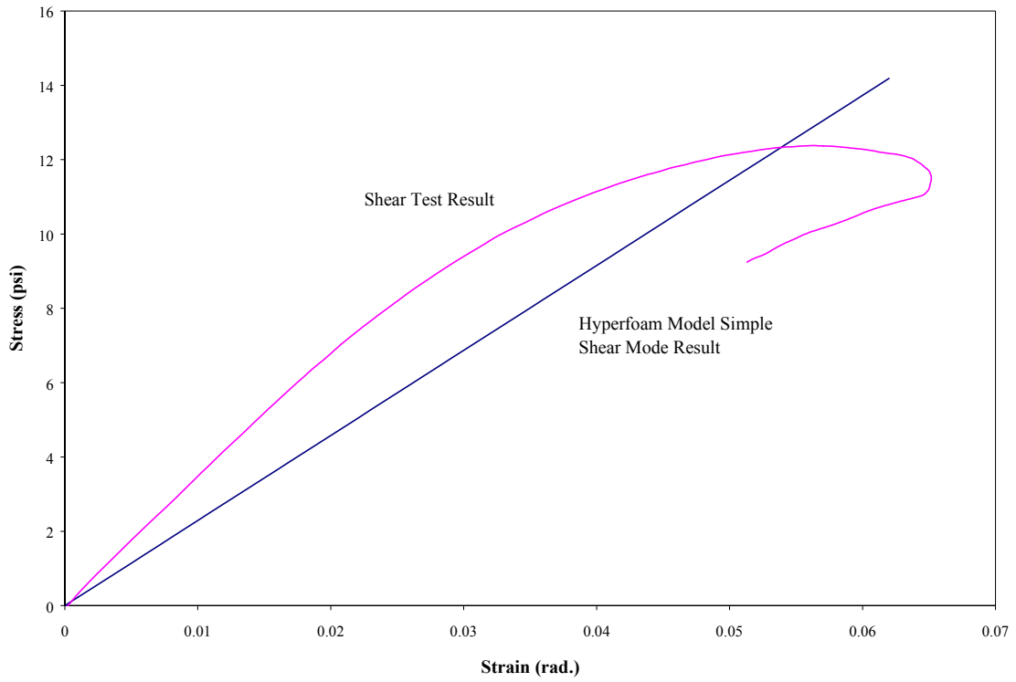
Fig. 4-12 Comparison of Stress-Strain Curves from Compression Test and Simple Shear Mode of Hyperfoam Model
