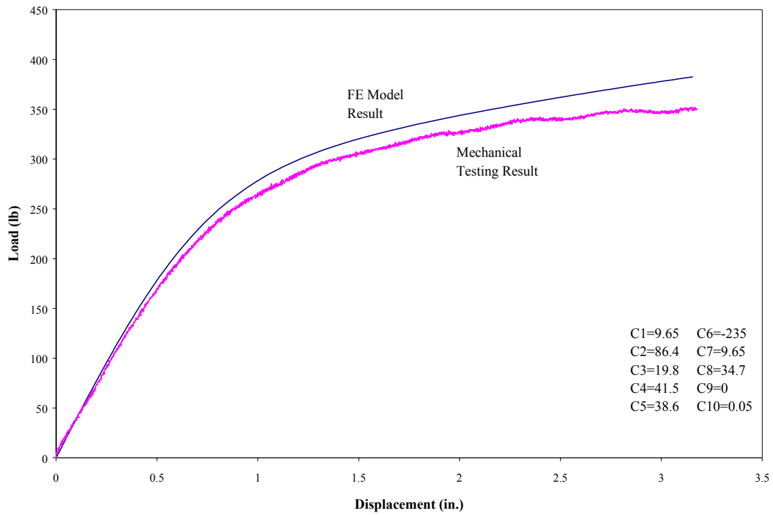
Fig. 4-27 Load-Displacement Curves of a 7 Foot Long Beam with 6 Foot Span and Load Applied at 1/3 of the Span (User-Supplied Material 2)
