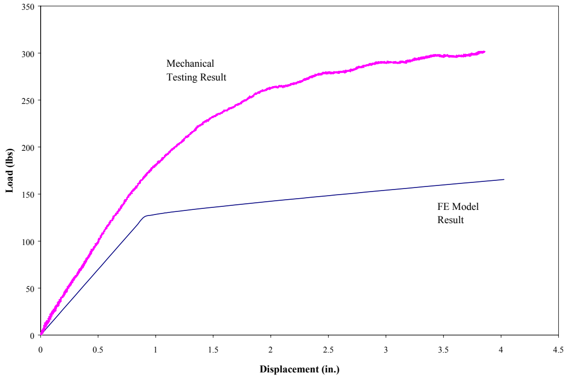
Fig. 4-19 Load-Displacement Curves for an 8 Foot Long Beam with 8 Foot Span and Load Applied at 1/3 of the Span (Bilinear Model)
