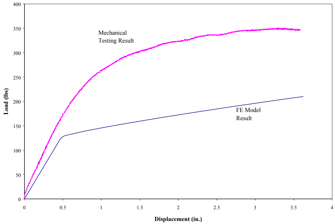
Fig 4-17 Load-Displacement Curves for a 7 Foot Long Beam with 6 Foot Span and Load Applied at 1/3 of the Span (Bilinear Model)
