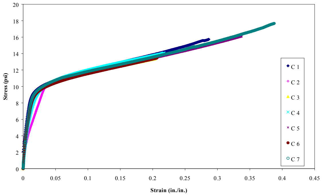
Fig. 4-1 Stress-Strain Curves for EPS in Compression
