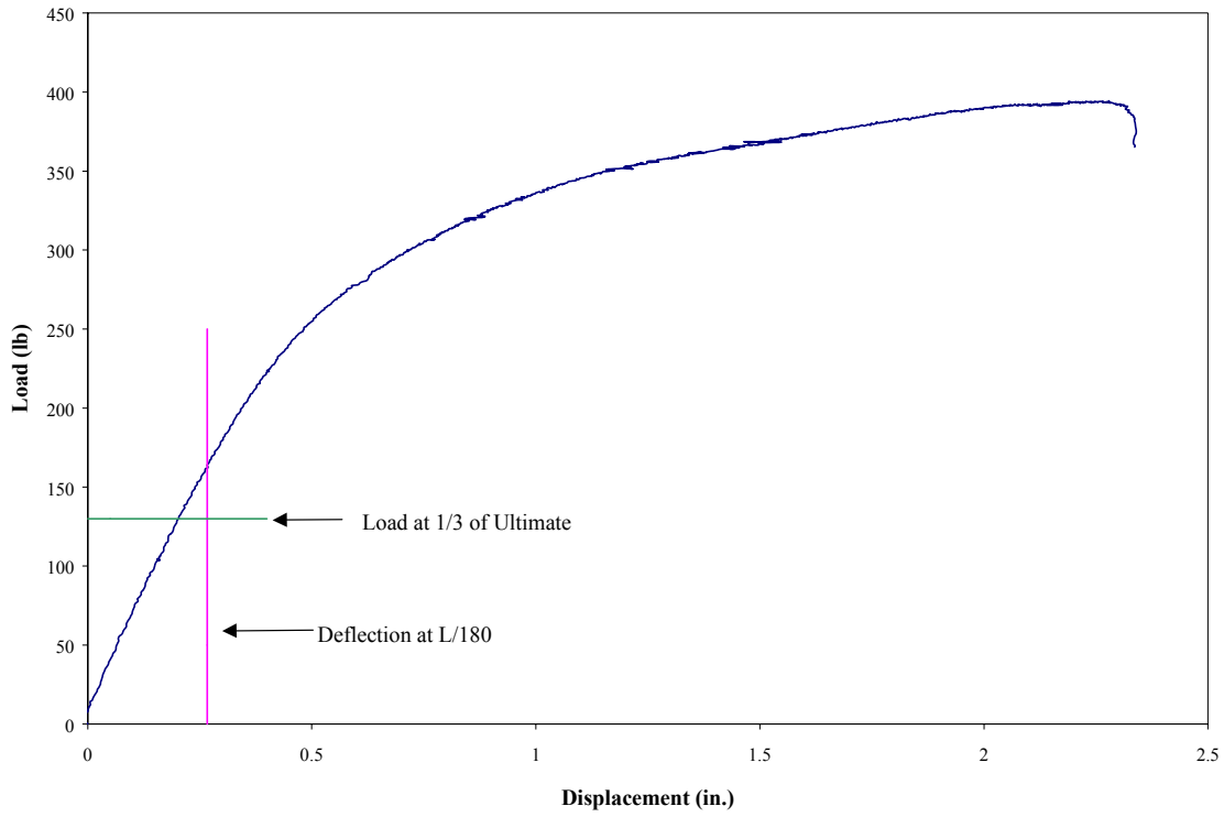
Fig. 5-5 Design Point for a 5 Foot Long Beam Provided by APA
