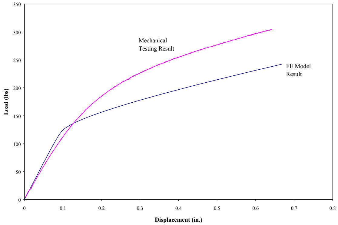
Fig. 4-15 Comparison of Load-Displacement Curves for a 3 Foot Long Beam with 2 Foot Span and Load Applied at 1/3 of the Span (Bilinear Model)
