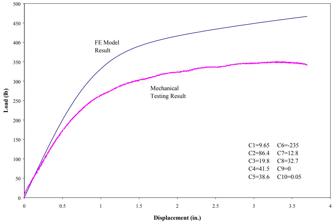
Fig. 4-23 Load-Displacement Curves of an 8 Foot Long Beam with 6 Foot Span and Load Applied at 1/3 of the Span (User-Supplied material 1)
