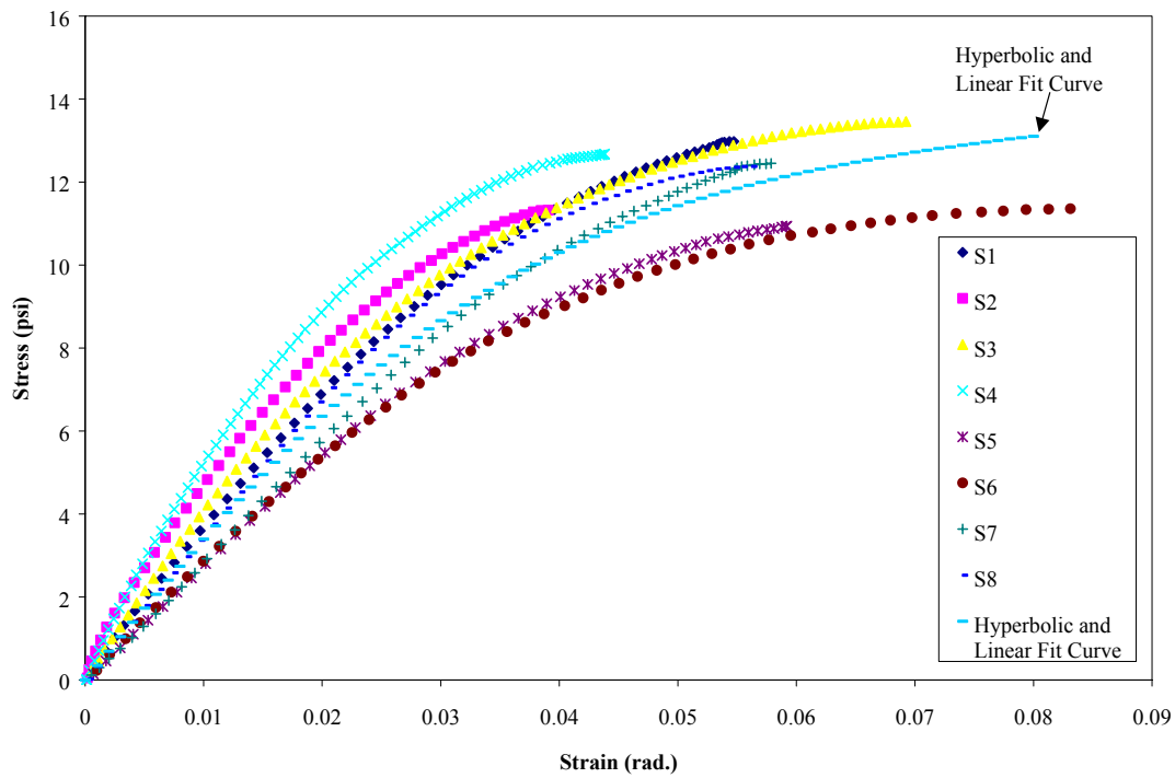
Fig. 4-8 Stress-Strain Curves for EPS in Shear between Testing & Hyperbolic and Linear Function Fit
