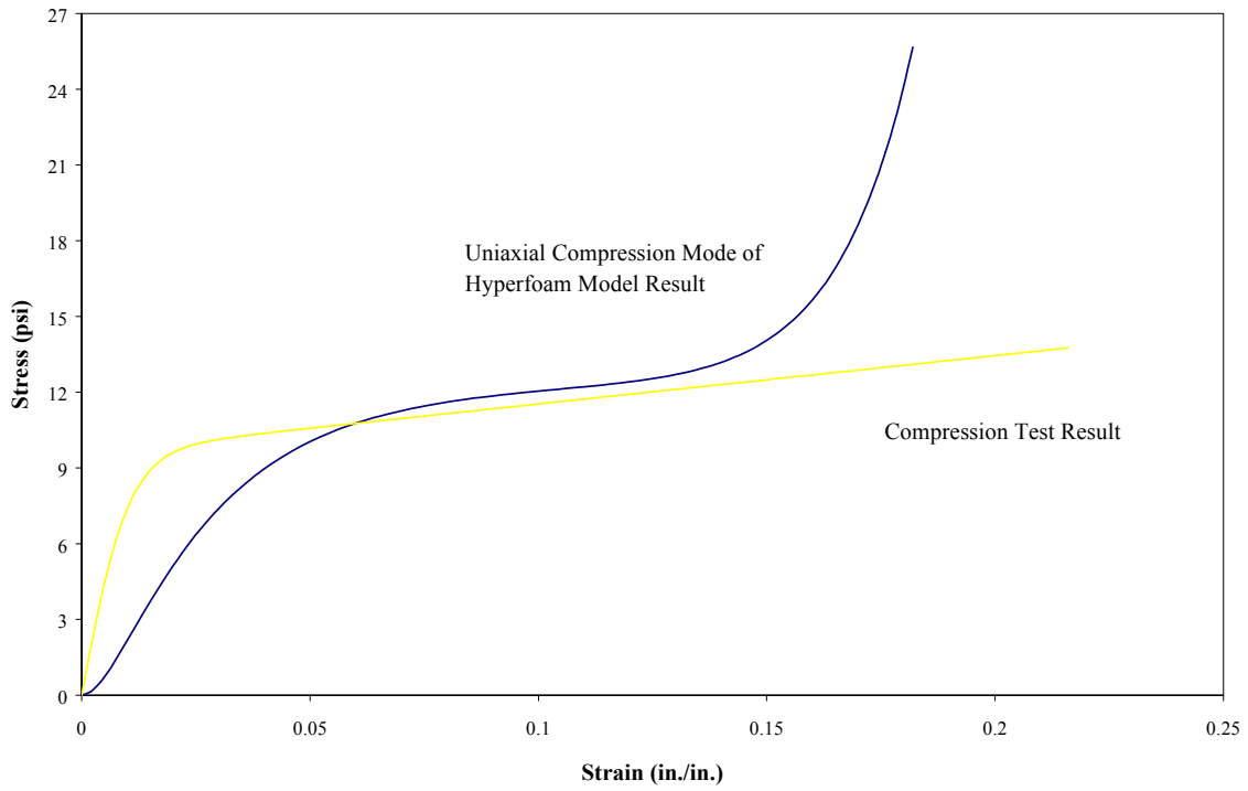
Fig. 4-11 Comparison of Stress-Strain Curves from Compression Test and Uniaxial Compression Mode of Hyperfoam Model
