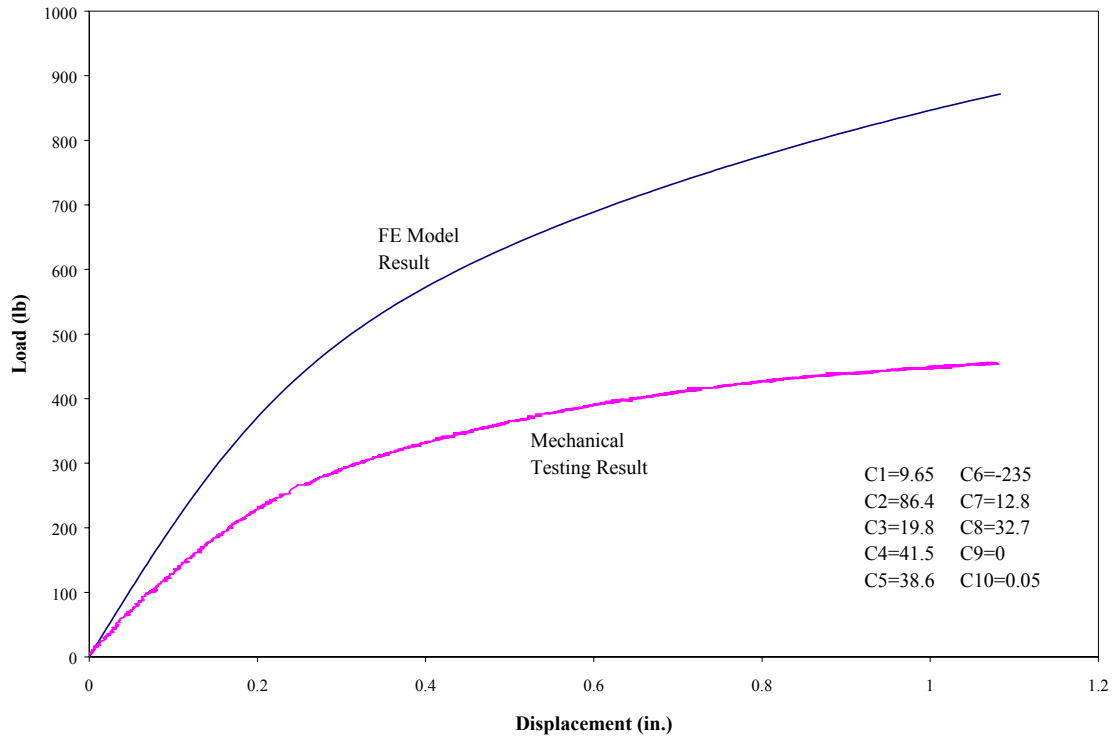
Fig. 4-20 Load-Displacement Curves for a 3 Foot Long Beam 2 Foot Span and Load Applied at 1/3 of the Span (User-Supplied Material 1)
