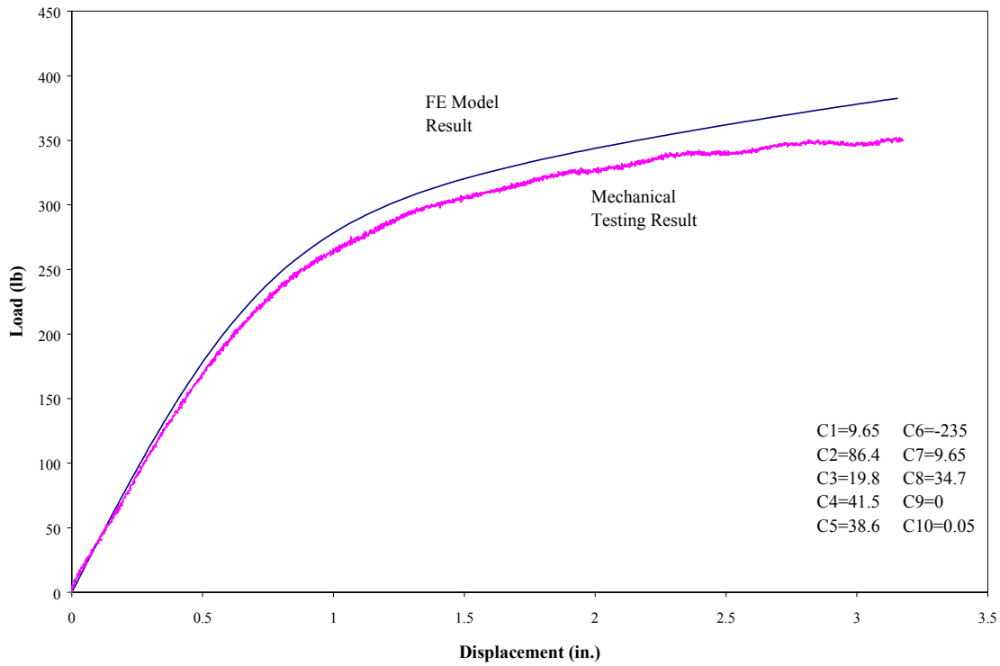
Fig. 4-22 Load-Displacement Curves of a 7 Foot Long Beam with 6 Foot Span and Load Applied at 1/3 of the Span (User-Supplied Material 1)
