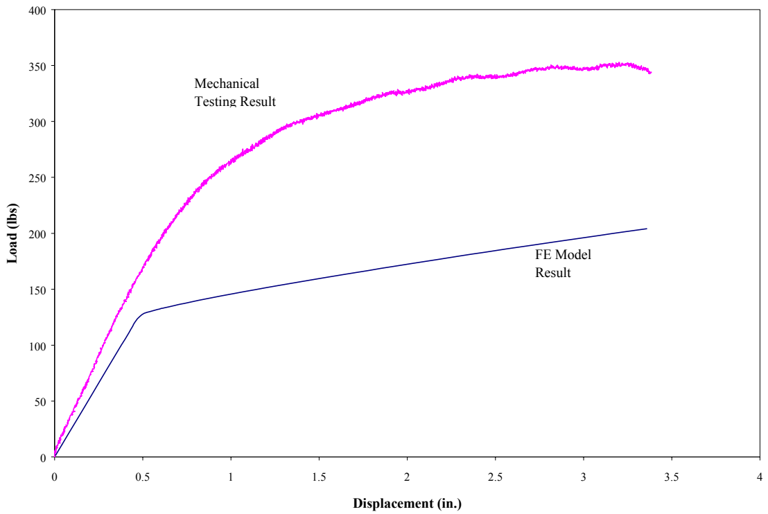
Fig. 4-18 Load-Displacement Curves for a 8 Foot Long Beam with 6 Foot Span and Load Applied at 1/3 of the Span (Bilinear Model)
