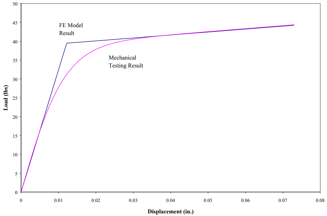
Fig. 4-13 Comparison of Load-displacement Curves of EPS in Compression from Mechanical Test and Bilinear Model
