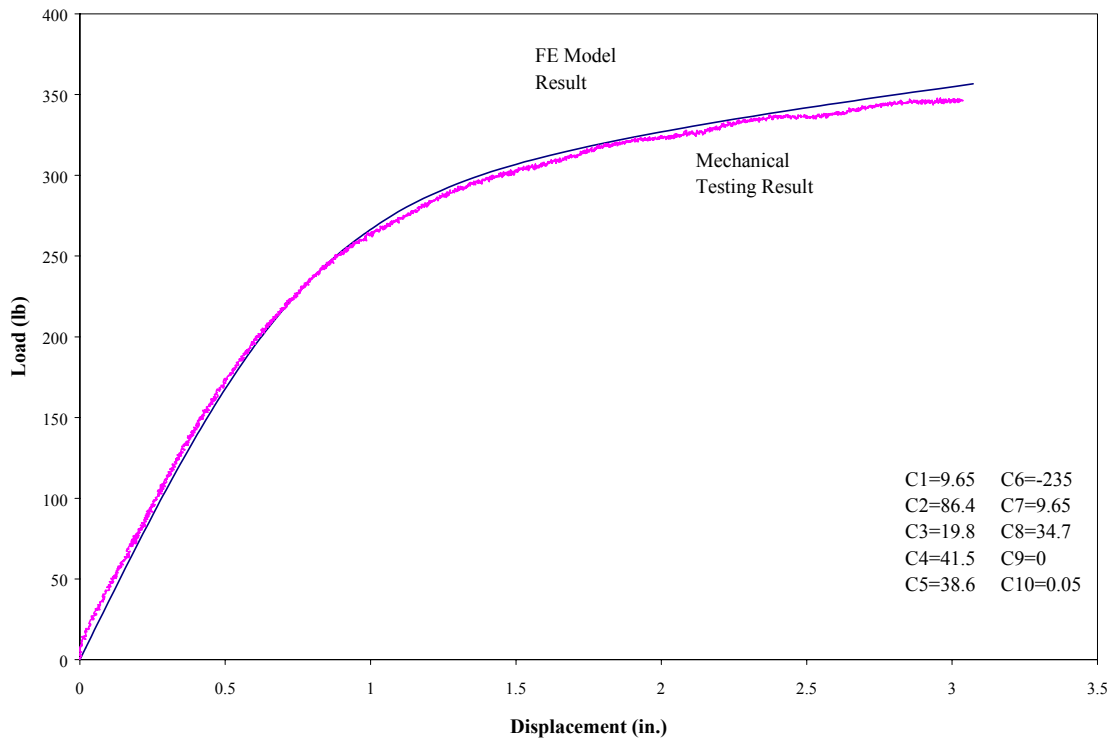
Fig. 3-28 Load-Displacement Curves of an 8 Foot Long Span with 6 Foot Span and Load Applied at 1/3 of the Span (User-Supplied Material 2)
