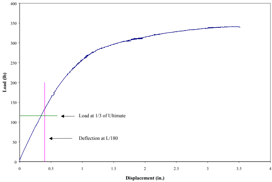
Fig. 5-6 Design Point for a 7 Foot Long Beam Provided by APA
