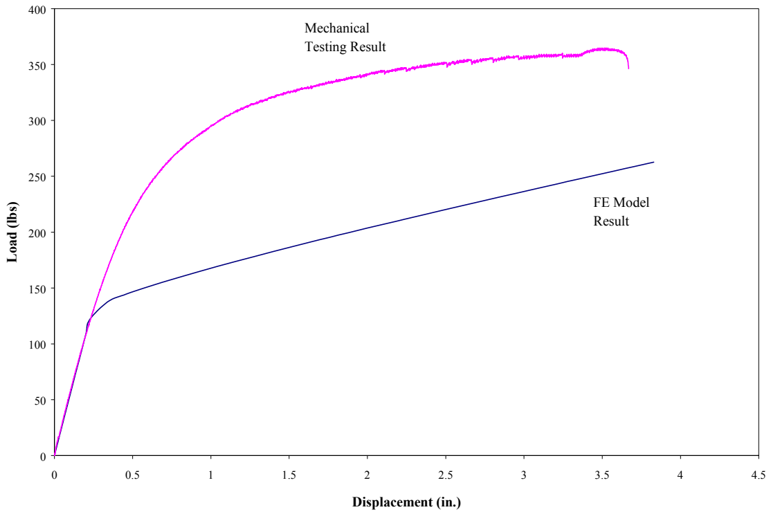
Fig. 4-16 Load-Displacement Curves for a 5 Foot Long Beam with 4 Foot Span and Load Applied at 1/3 of the Span (Bilinear Model)
