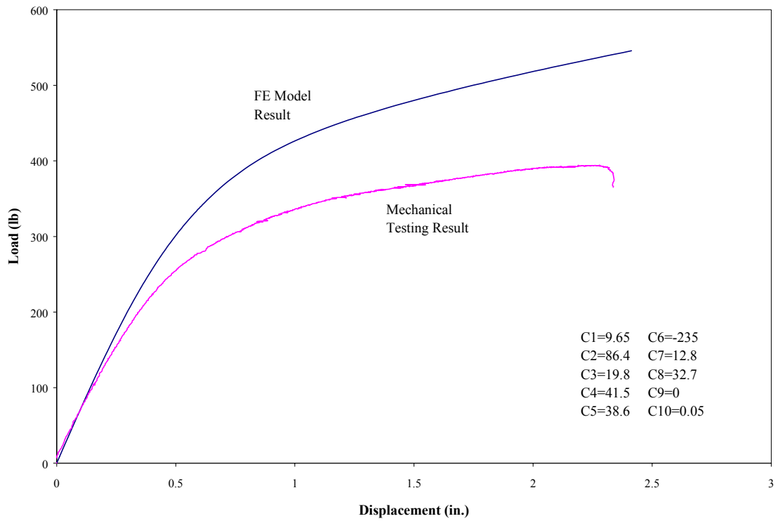
Fig. 4-21 Load-Displacement Curves for a 5 Feet Long Beam with 4 Feet Span and Load Applied at 1/3 of the Span (User-Supplied Material 1)
