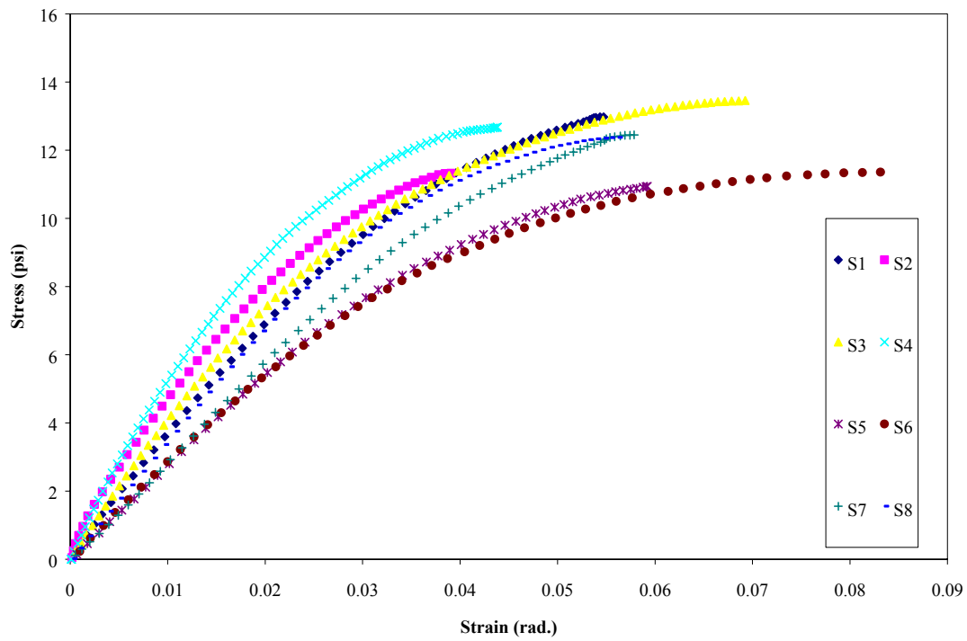
Fig. 4-7 Stress-Strain Curves for EPS in Shear
