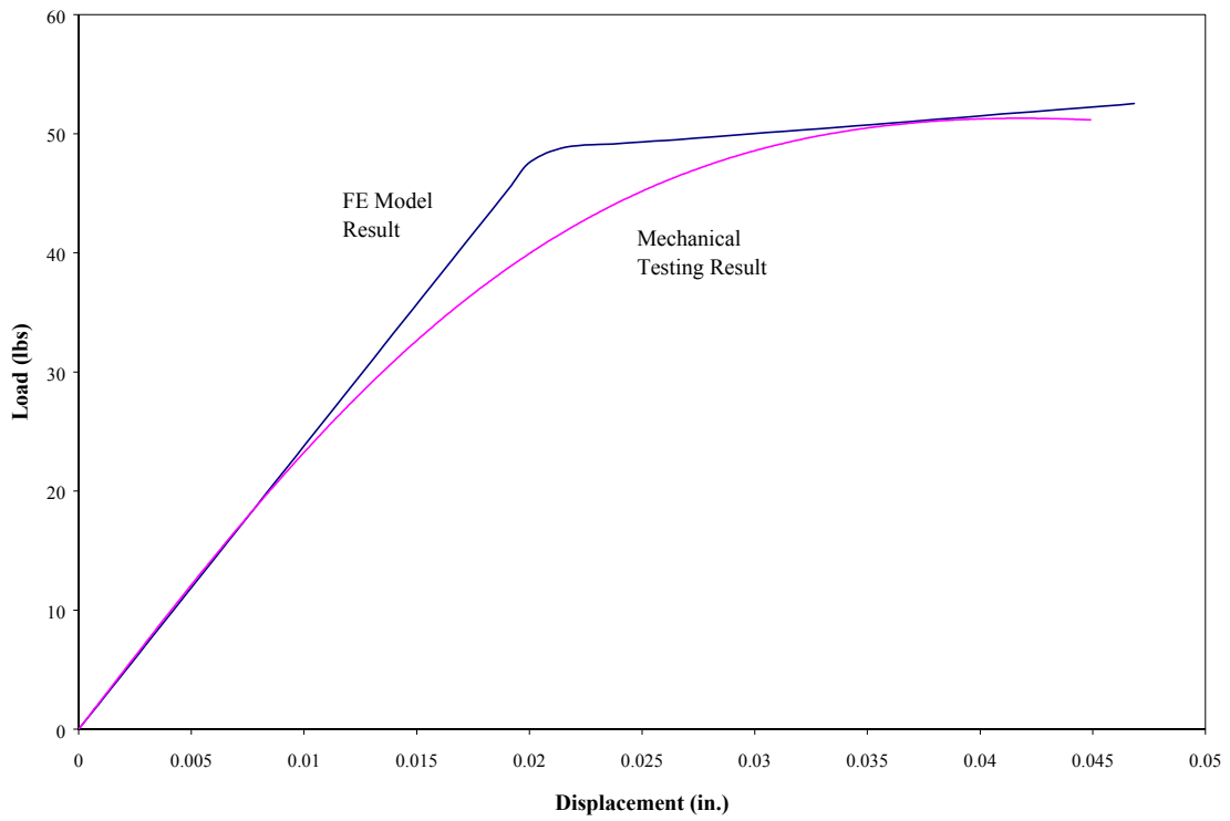
Fig. 4-14 Comparison of Load-displacement Curves of EPS in Tension from Mechanical Test and Bilinear Model
