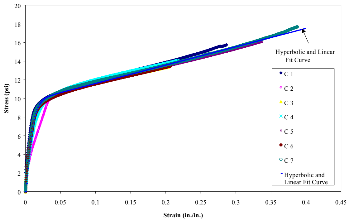
Fig. 4-2 Stress-Strain Curves for EPS in Compression between Testing & Hyperbolic and Linear Function Fit
