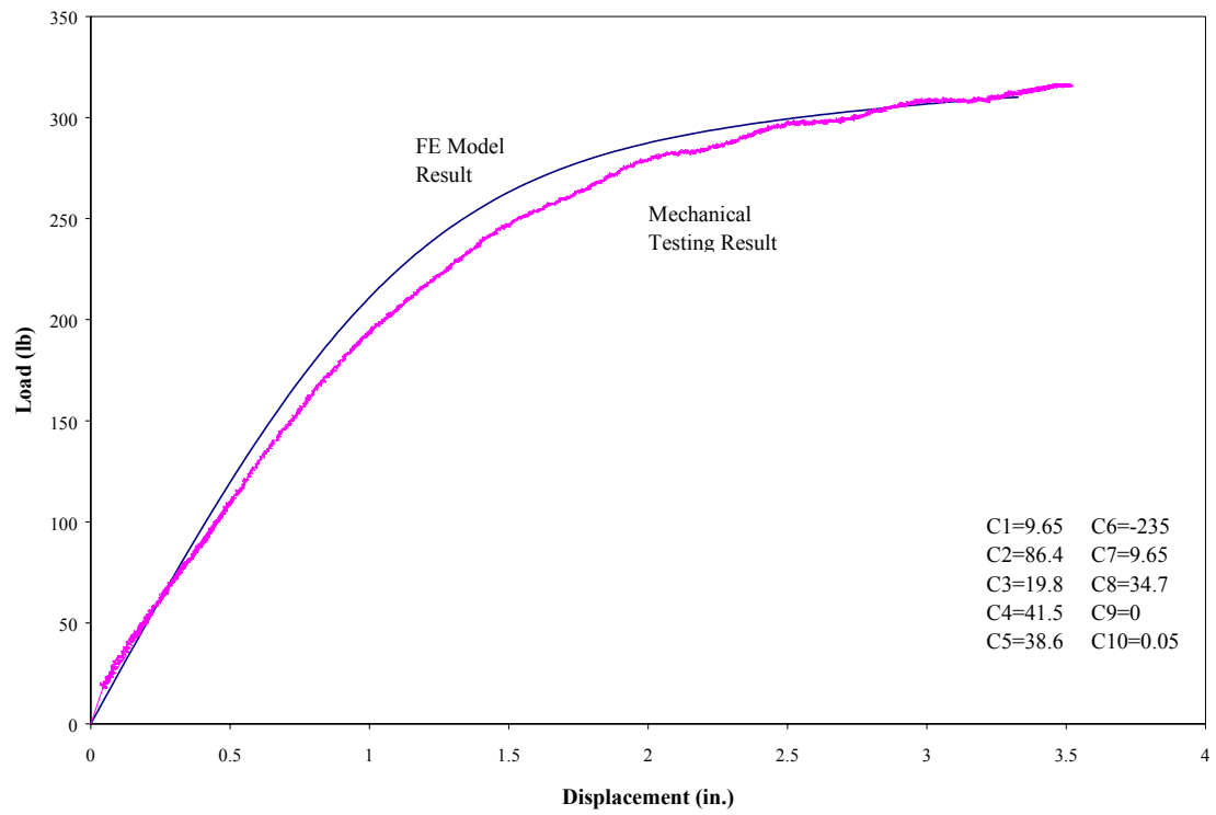
Fig. 4-29 Load-Displacement Curves of an 8 Foot Long Beam with 8 Foot Span and Load Applied at 1/3 of the Span (User-Supplied Material 2)
