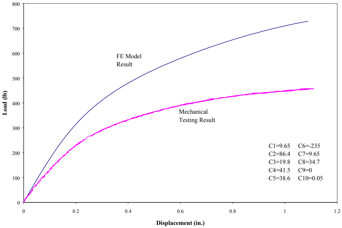
Fig. 4-25 Load-Displacement Curves of a 3 Foot Long Beam with 2 Foot Span and Load Applied at 1/3 of the Span (User-Supplied Material 2)
