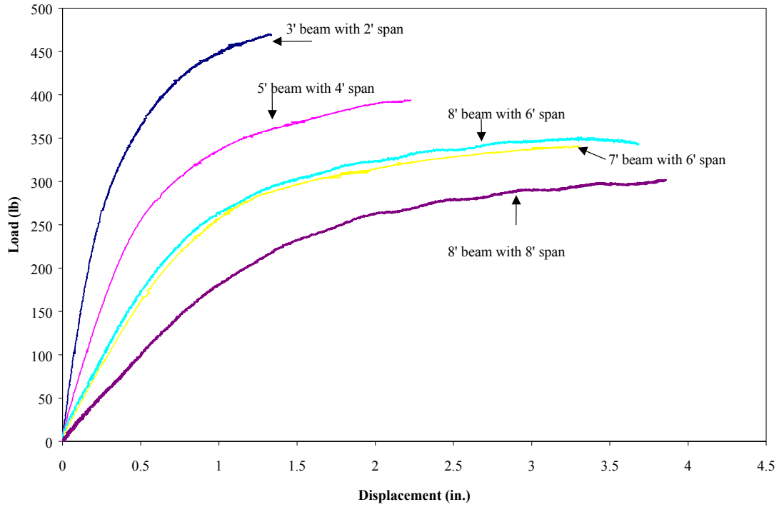
Fig. 4-9 Load-Displacement Curve for SIP Beams with Various Span
