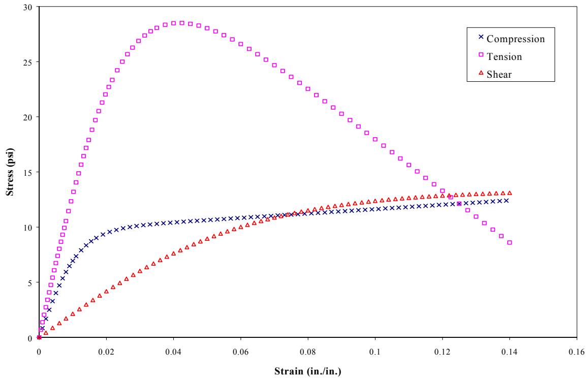
Fig. 5-1 EPS Compression, Tension, and Shear Stress-Strain Curves
